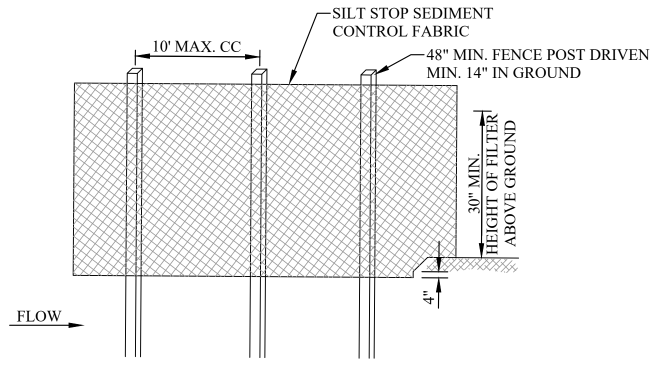
SILT FENCE NOT TO SCALE
