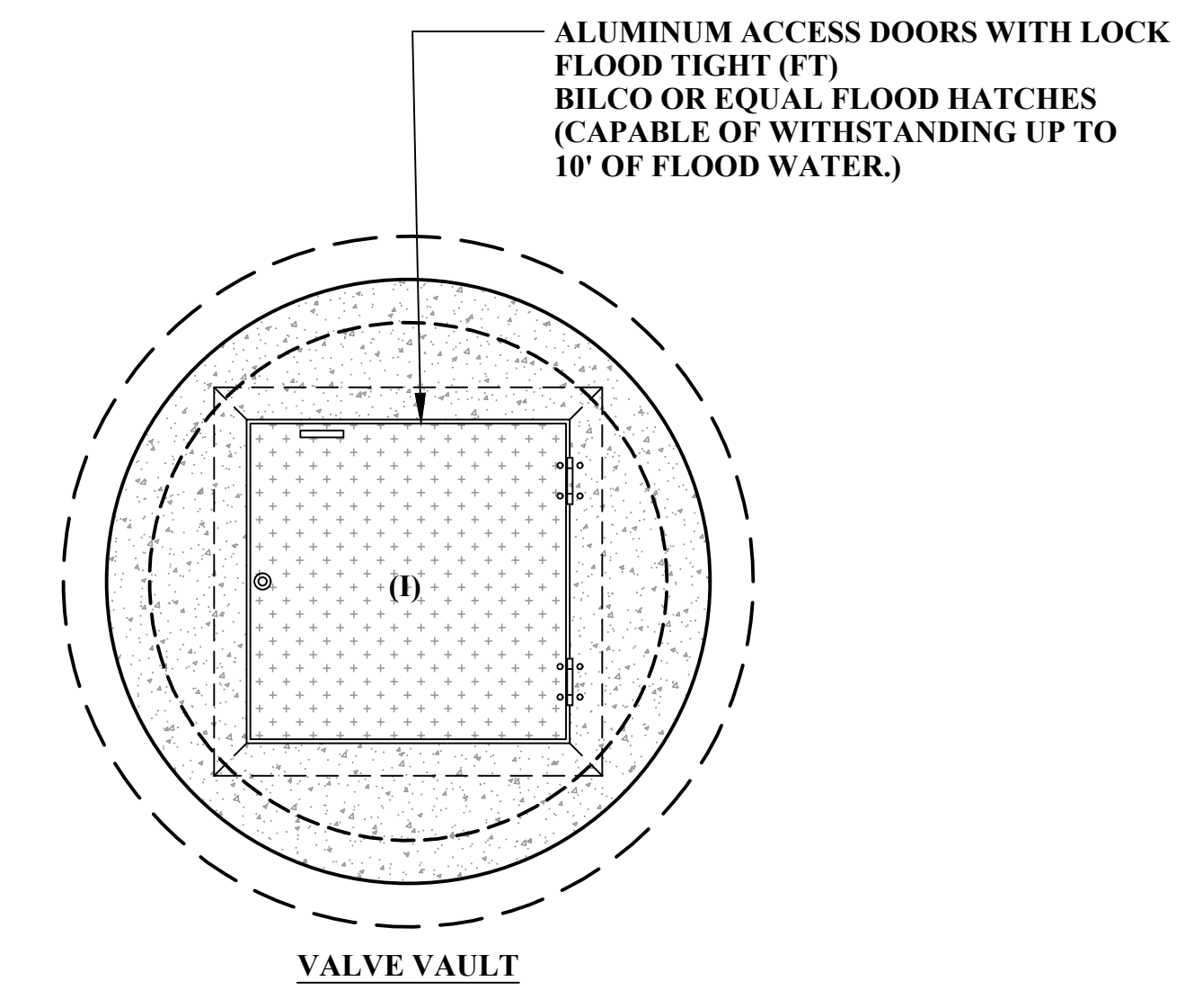
PLAN VIEW
