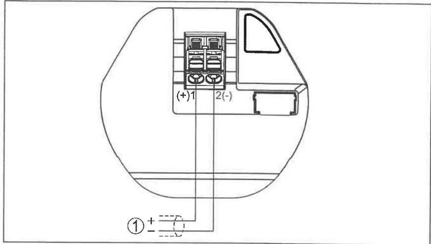
Fig. 18: Connection compartment VEGAPULS 21
