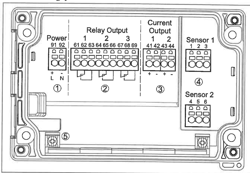
Fig. 6: Wiring plan VEGAMET 842
