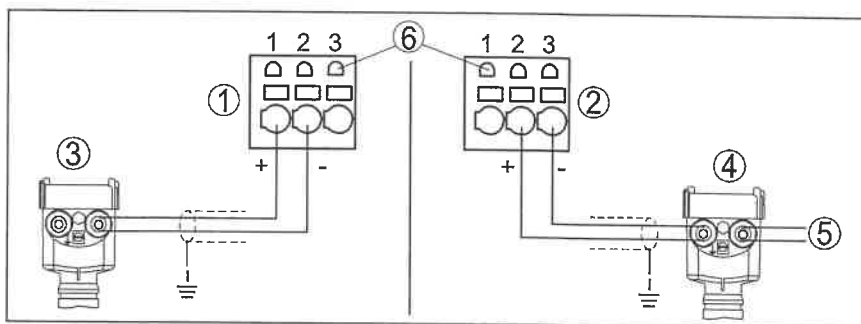
Fig. 7: Sensor input 1 for two-wire/four-wire sensor (active/passive)
